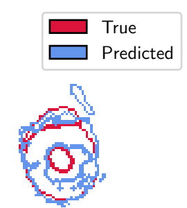
segmentations
